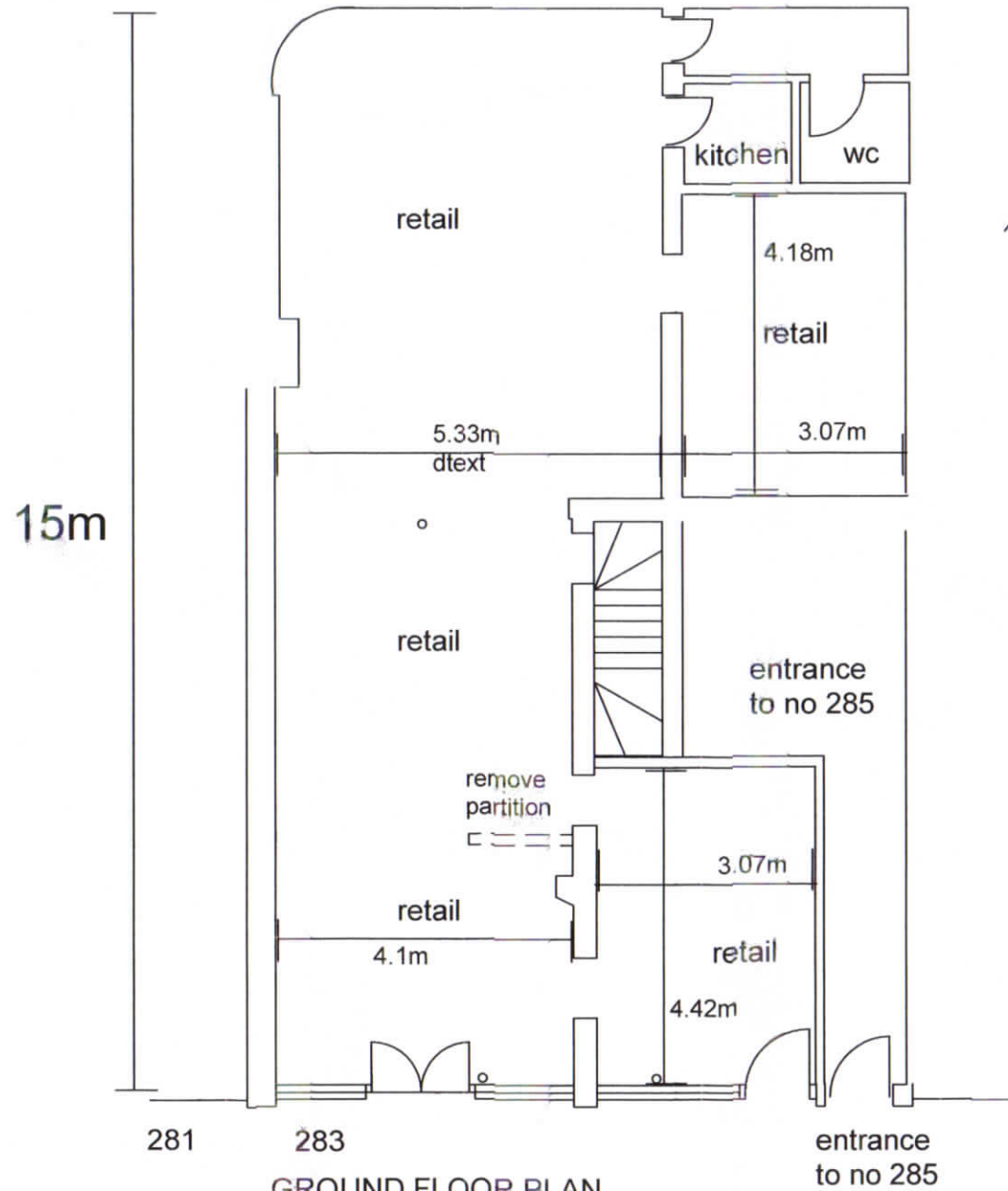
GROUND FLOOR PLAN PROPOSED
